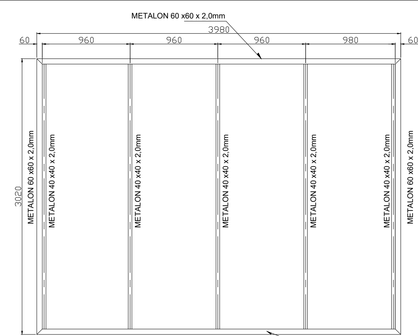
VISTA FRONTAL
